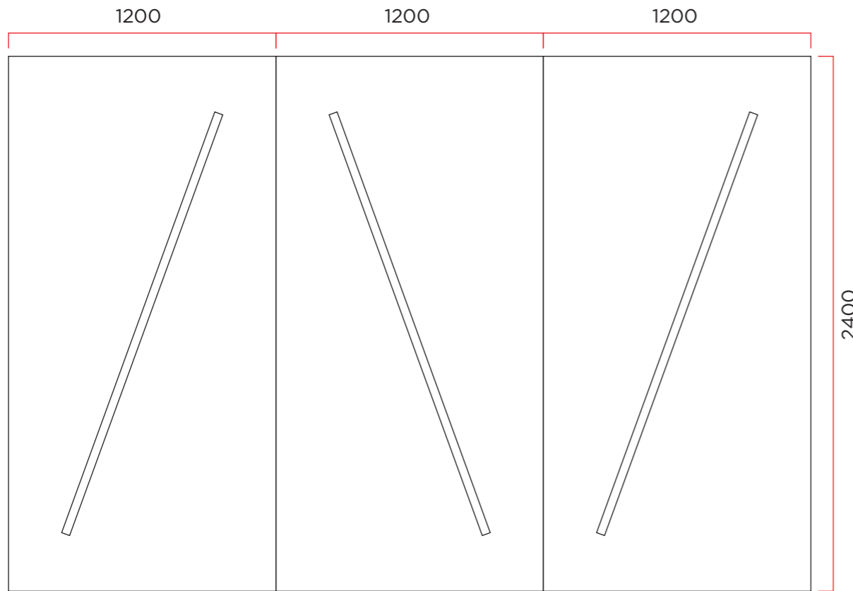
G1 Lights 2005x25mm
